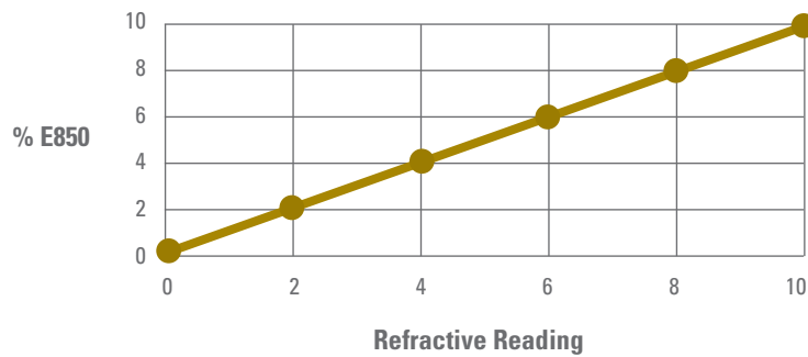
Concentration vs Refractive Index
